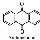
Anthrachinon
