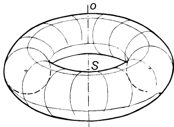
Anuloid
